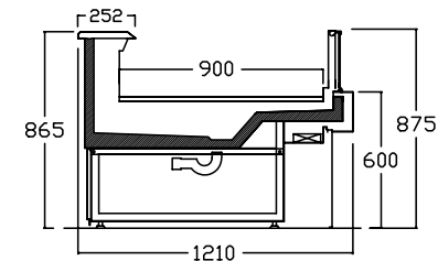
NEVA121 DÜZ DEVİRME CAM SELF NEVA121 FLAT UP-DOWN SELF
