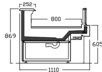
NEVA111 DÜZ DEVİRME CAM SELF NEVA111 FLAT UP-DOWN SELF
