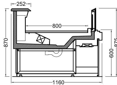
NEVA116 DÜZ-3-S BAZALI NEVA116 FLAT-3-S COVERED BASE
