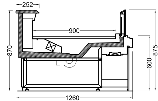
NEVA126 DÜZ-3-S BAZALI NEVA126 FLAT-3-S COVERED BASE
