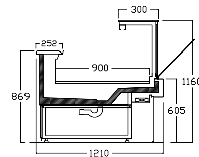
NEVA121 DÜZ DEVİRME CAM NEVA121 FLAT UP-DOWN GLASS
