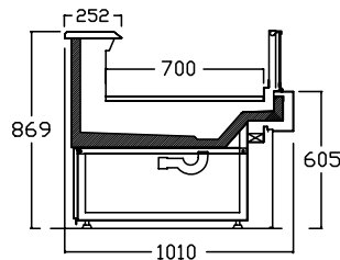
NEVA101 DÜZ DEVİRME CAM SELF NEVA101 FLAT UP-DOWN SELF
