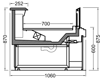
NEVA106 DÜZ-3-S BAZALI NEVA106 FLAT-3-S COVERED BASE
