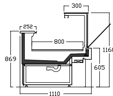
NEVA111 DÜZ DEVİRME CAM NEVA111 FLAT UP-DOWN GLASS
